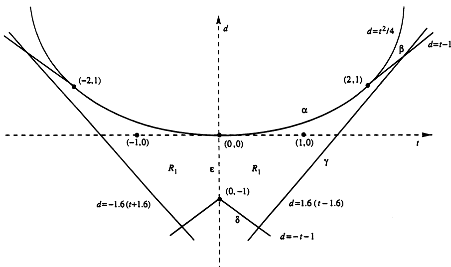
FIGURE 3.7. The set R_1 in the variables (t, d) .
