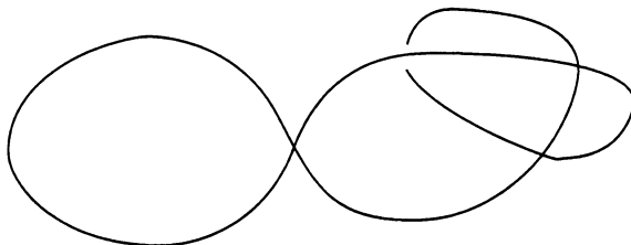
FIGURE A.1. The space W .
